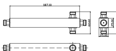
3 way Splitter:
