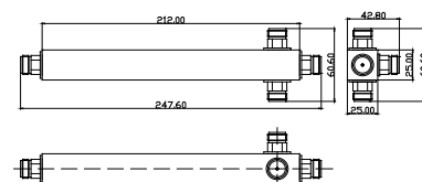
4 way Splitter:
