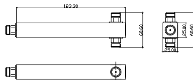
2 way Splitter:
